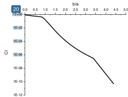
Figure 8: The capsizing index correspond to the index "b/a" of weather criterion with damping factor based on weather criterion
