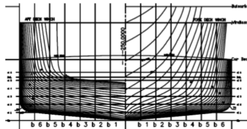
Figure 1: The body plan of subject ship
